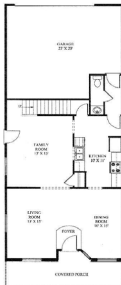
2 story—Finished living area 1985 sq. ft.
